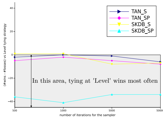
Fig. 5 Win/loss plot of each combination of (flagship classifier) \times (S or SP tying strategy) versus tying at level (L).
